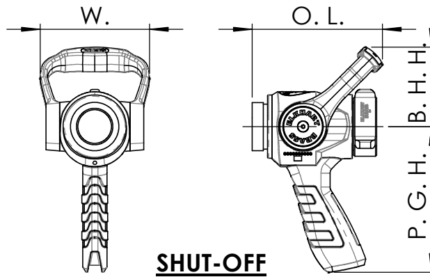
XD SHUT-OFF DIMENSIONAL TABLE
